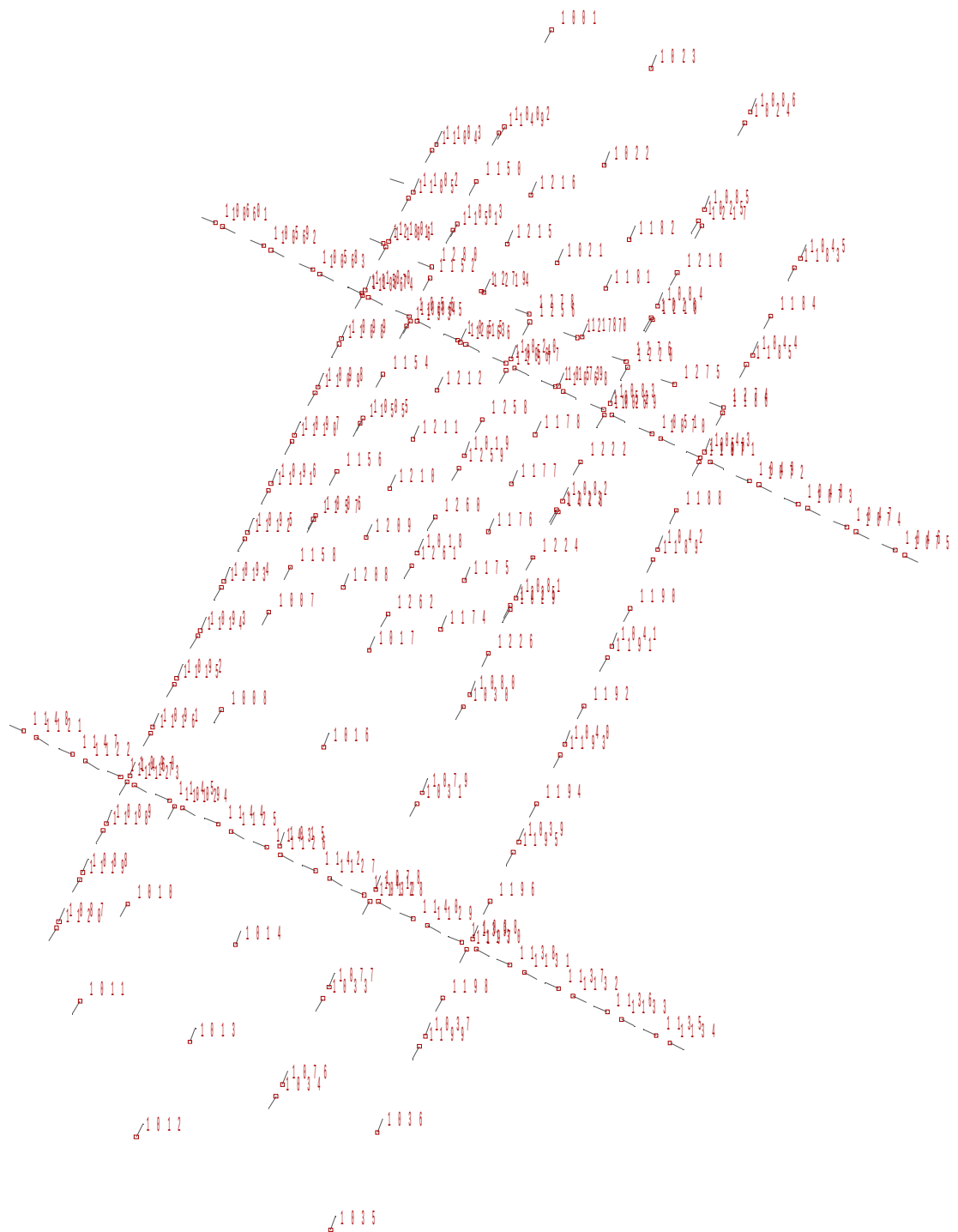
Figure 5 - Complete block of IGI photo flight (horizontal and vertical residuals, small vectors indicating flight direction).
